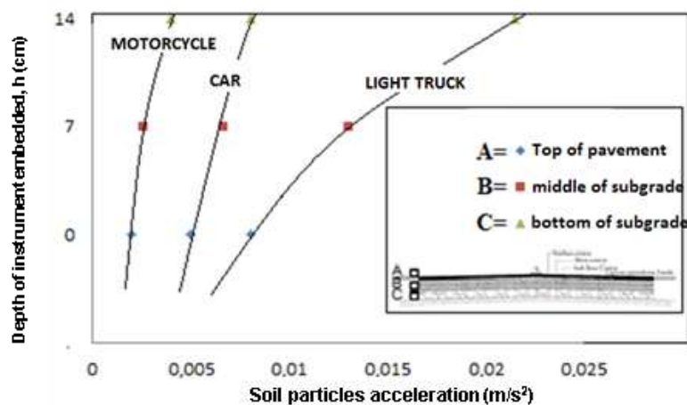
Figure 8. Soil particles acceleration due to traffic load based on type of vehicles
