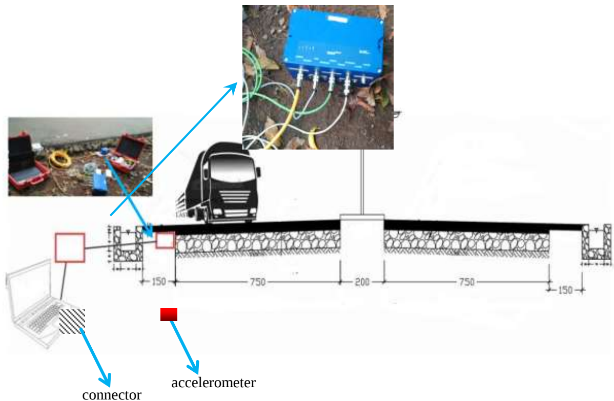
Figure 2. Installation of seismic monitoring unit during field investigation
