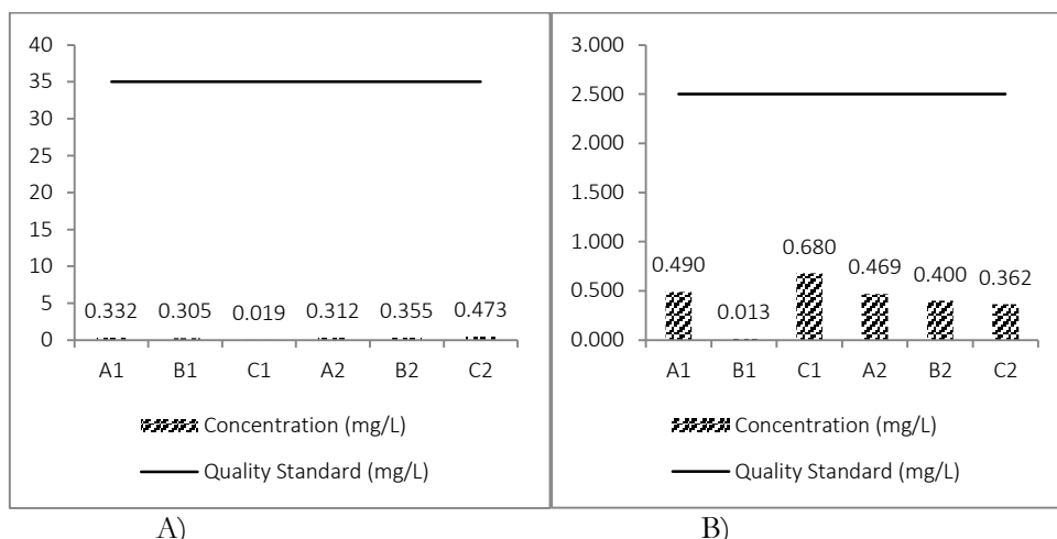
Figure 3 Comparison graph of concentration value of A) barium and B) chromium on Toxicity Characteristic Leaching Procedure test to quality standard.
