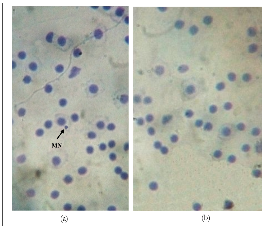
Figure 1. Peripheral blood film of catfish, C. gariepinus , showing (a) the manifestation of micronucleus (MN) and (b) normal erythrocyte.
