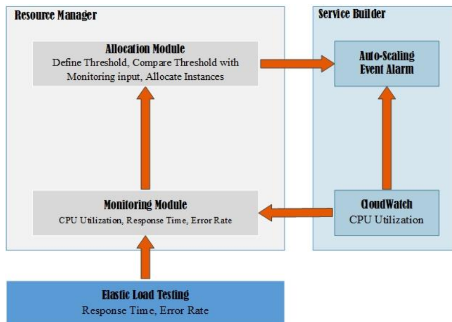
Figure 4. Resource manager
