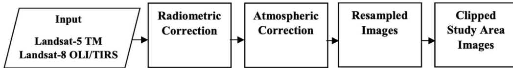
Figure 2. Image preprocessing steps.
