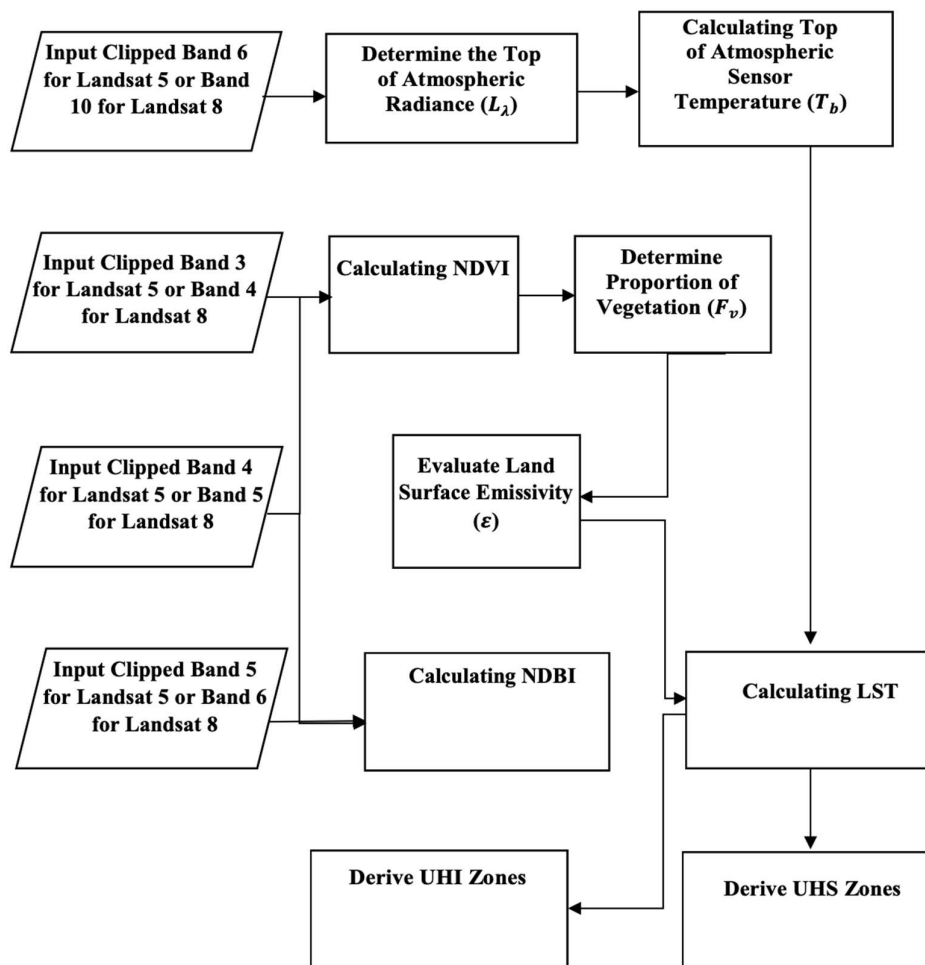
Figure 3. Flowchart for NDVI, NDBI, LST UHI and UHS zones derivation.
