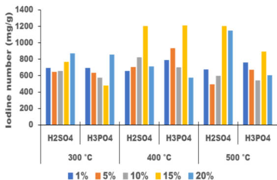
Figure 5. The iodine number of activated carbon
