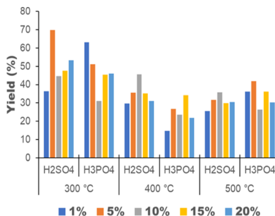
Figure 2. The yield of activated carbon
