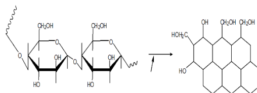
Figure 1. Carbonization reaction (Johannes, 2011)
