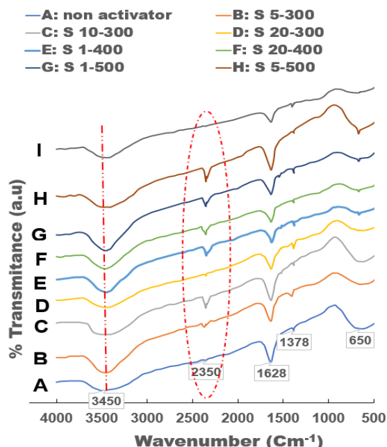
Figure 7. FTIR spectra of activated carbon by H 2 SO 4 activator in various activation temperature
