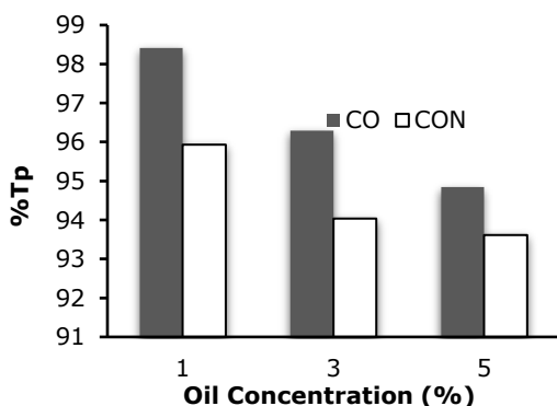
Figure 5. %Tp values of citronella oil (CO) and citronella oil nanoemulsion (CON)
