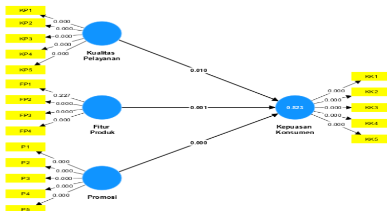
Figure 2. Hypothesis Testing
